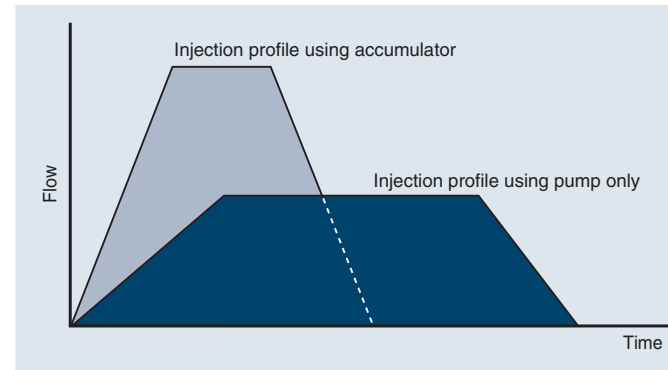
Cycle time reduction by using an accumulator
