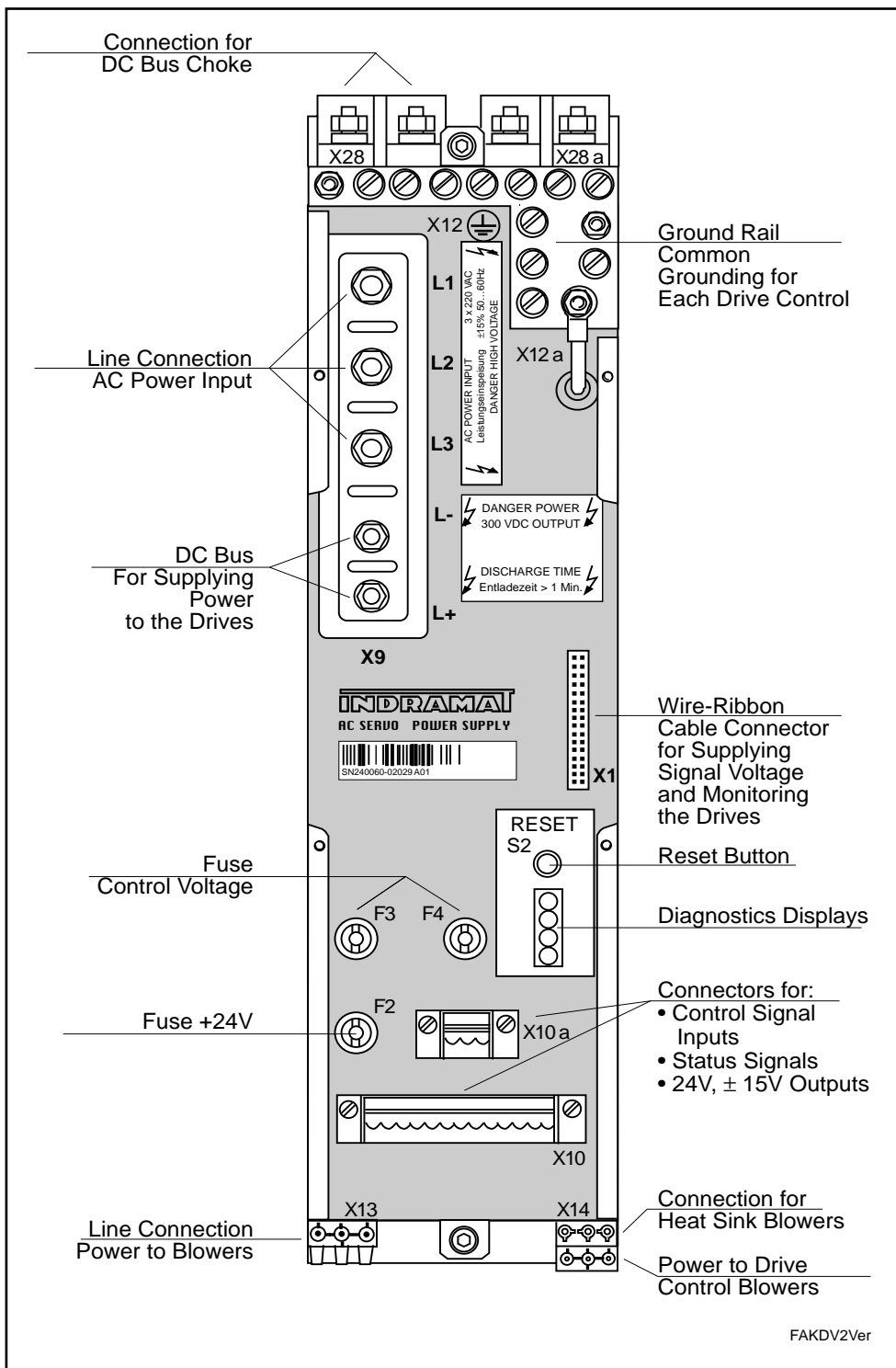
Fig. 2.15. Front view of KDV 2.3 supply module.
